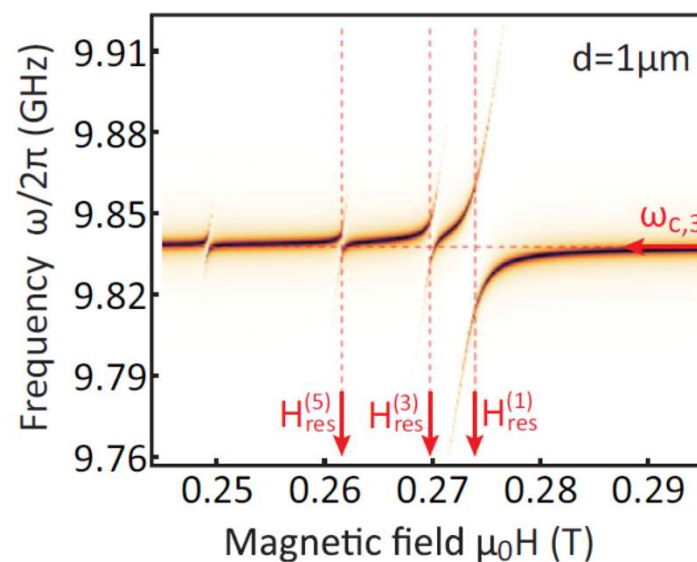
Calculated spin wave resonances of a YIG film with thickness d in a planar microwave cavity.
